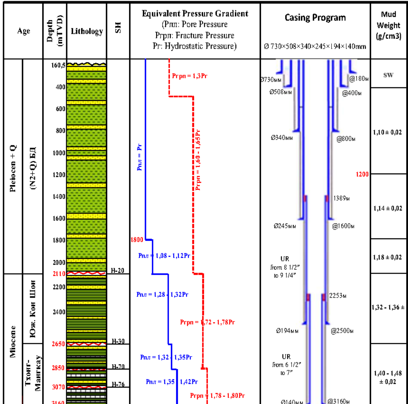
COMBINED PRESSURE GRAPH of THE WELL # TU-9 BLOCK 04-3. (TVD)
