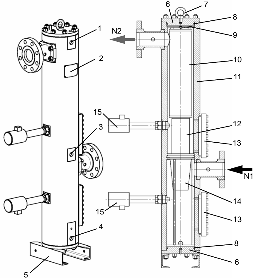
Fig. 5-1 Overview of assembly groups
