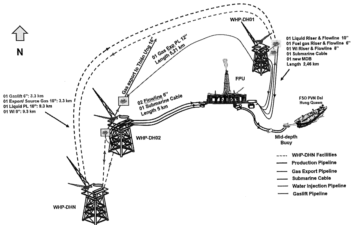
Figure 1.2: DAI HUNG NAM FIELD: FPU + FSO + WHP-DH01+ WHP-DH02+WHP DHN
