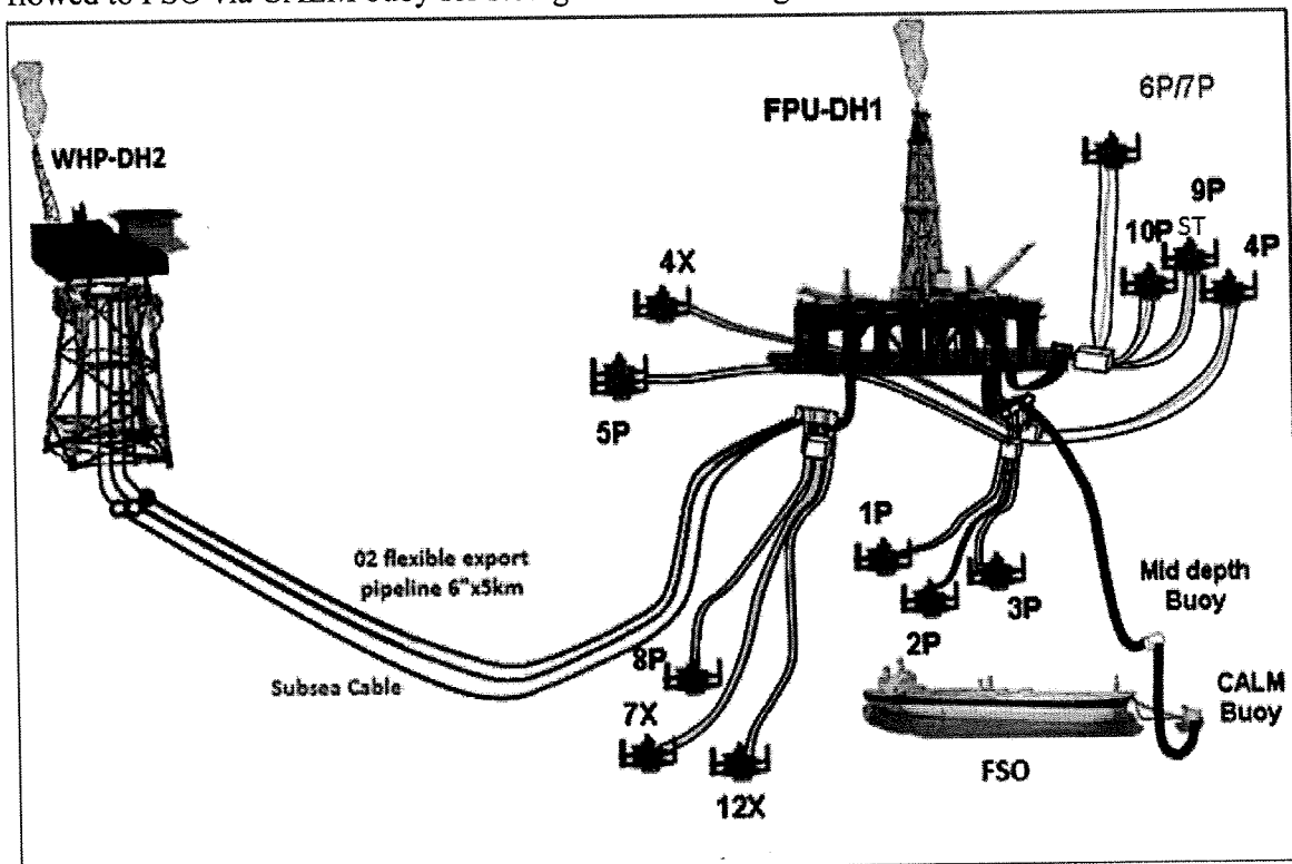
General Layout of Dai Hung Terminal
