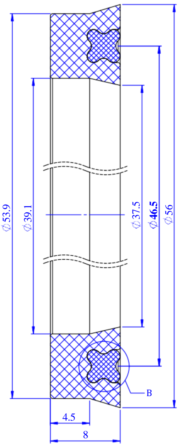
Rod seal - STD profile s8xOD53.9xID39.1
