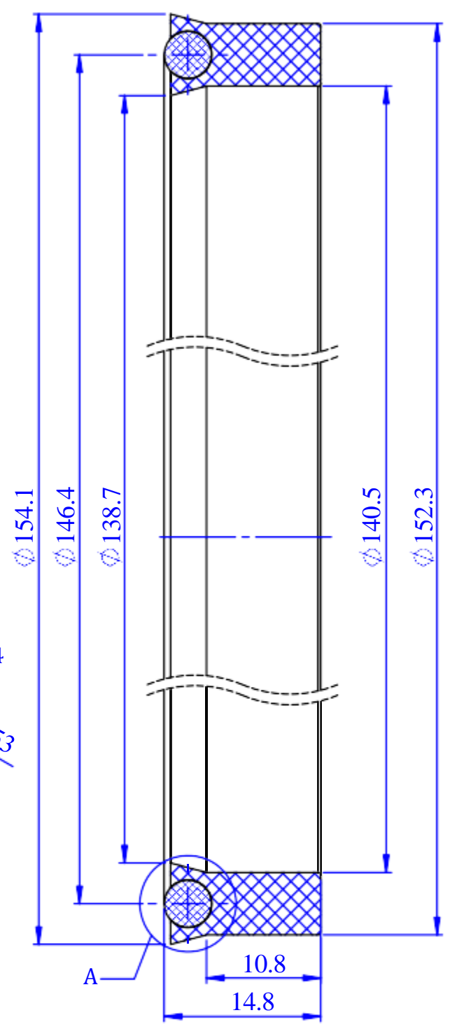
Piston seal - K21-P s14.2xOD152.3xID140.5
