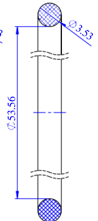
O-ring CS3.53xID53.56
