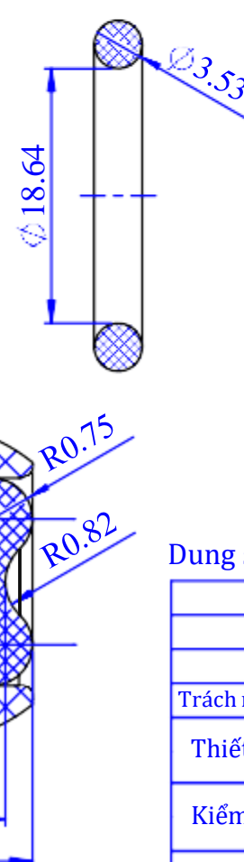
O-ring CS3.53xID18.64
