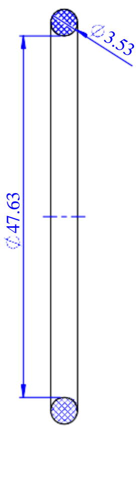
O-ring CS3.53xID47.63
