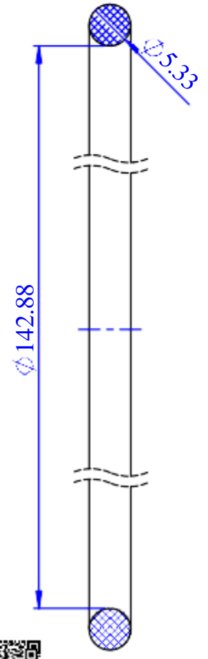
O-ring CS5.33xID142.88
