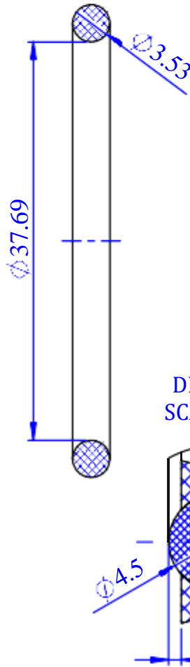
O-ring CS3.53xID37.69
