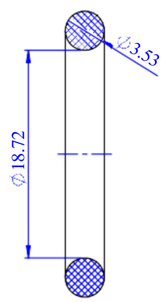
O-ring CS3.53xID18.72
