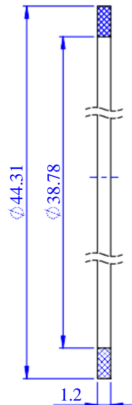
Back-up ring s1.2xOD44.31xID38.78
