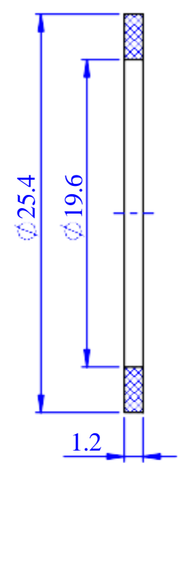
Back-up ring s1.2xOD25.4xID19.6
