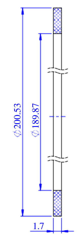
Back-up ring s1.7xOD200.53xID189.87
