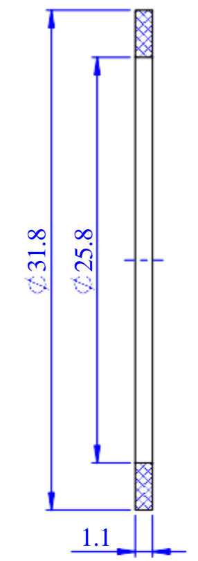
Back-up ring s1.1xOD31.8xID25.8
