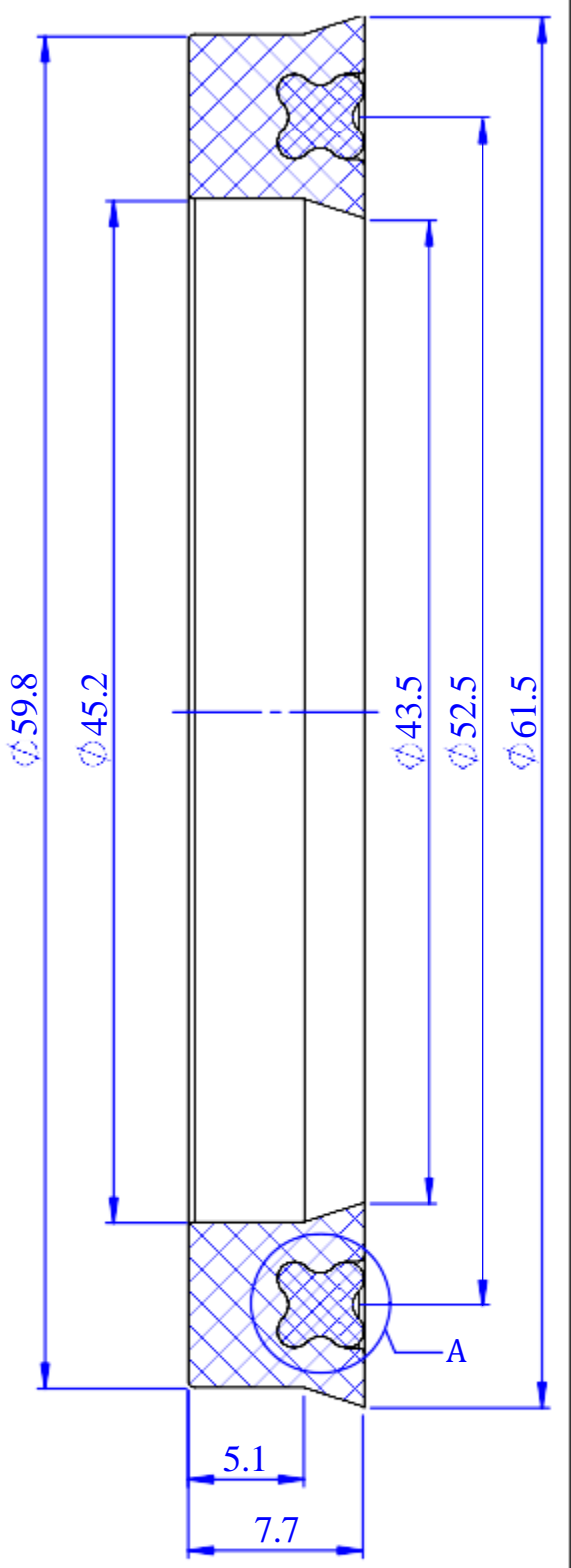
Rod seal - STD profile s7.7xOD59.8x ID45.2
