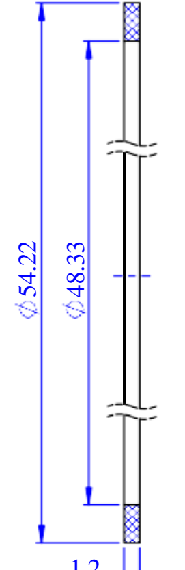
Back-up ring s1.2xOD54.22xID48.33
