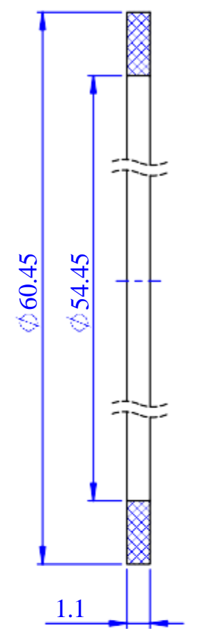
Back-up ring s1.1xOD60.45xID54.45
