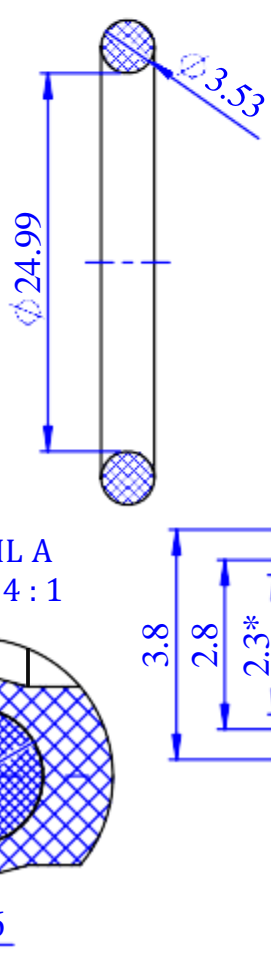
O-ring CS3.53xID24.99
