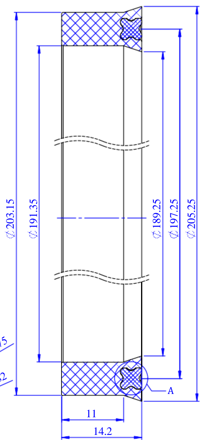
Piston seal - STD profile s14.2xOD203.15x ID191.35
