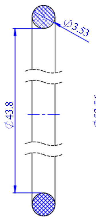
O-ring CS3.53xID43.8
