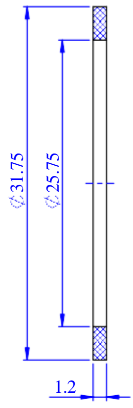
Back-up ring s1.2xOD31.75xID25.75
