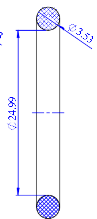
O-ring CS3.53xID24.99
