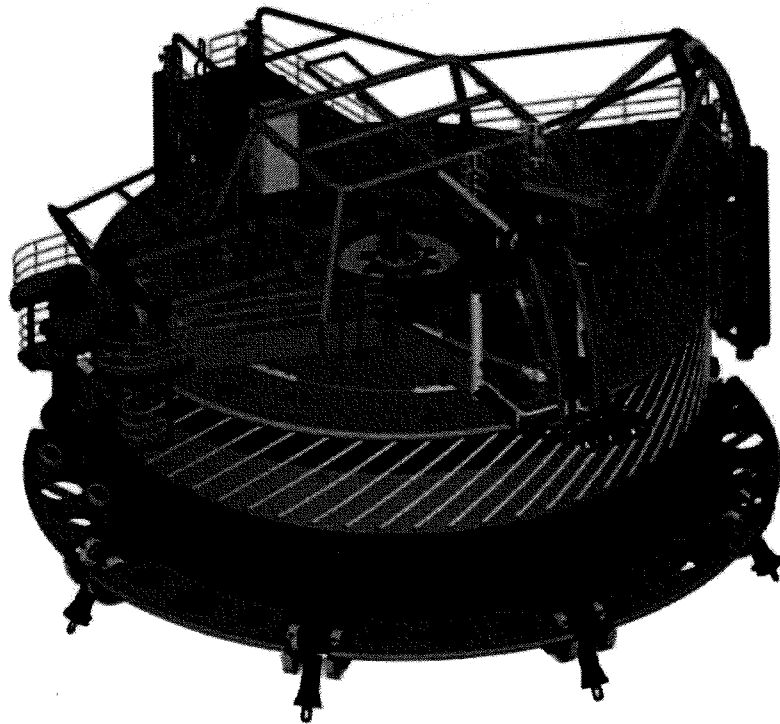
Figure 3: 3D general layout of CALM buoy Dai Hung
