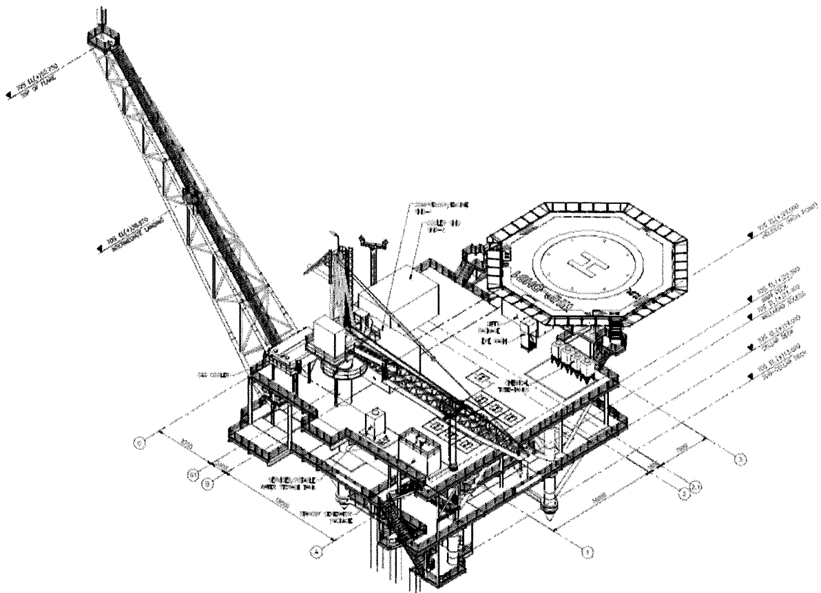
Figure 4 : Configuration of WHP-DH1 Topside
