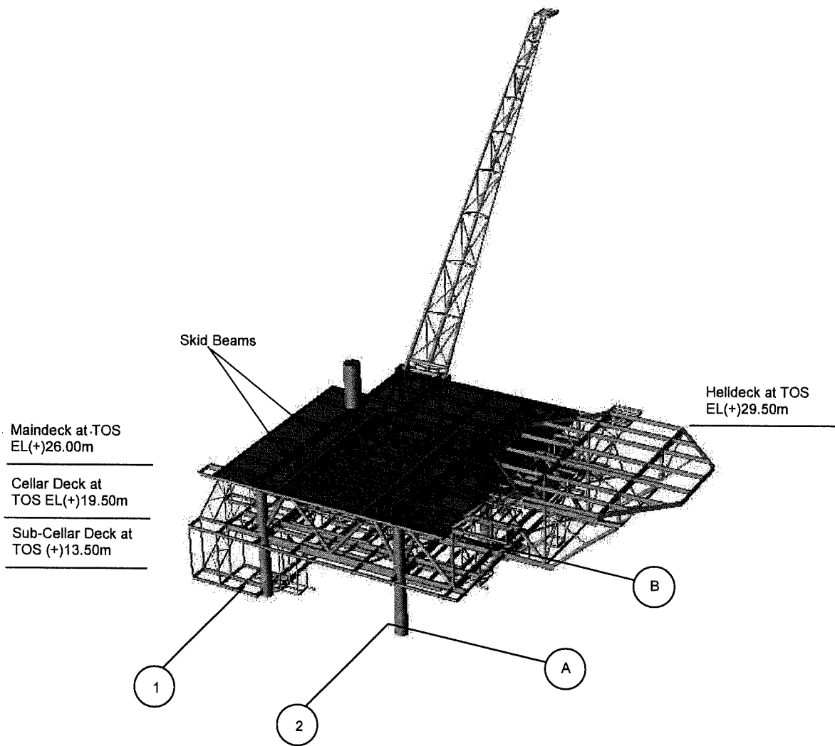
Figure 1 : Configuration of WHP-DH2 Topside
