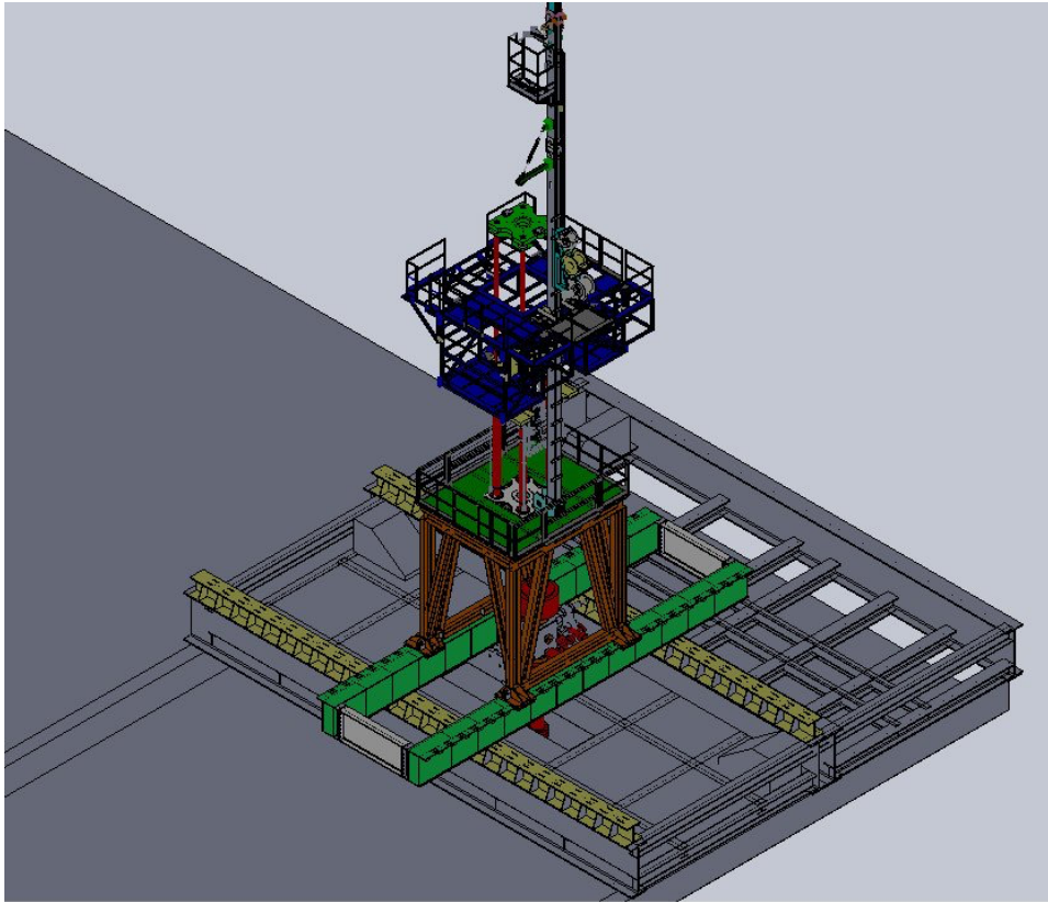
Fig 1: Layout equipment on upper deck of Platform (for reference only)
