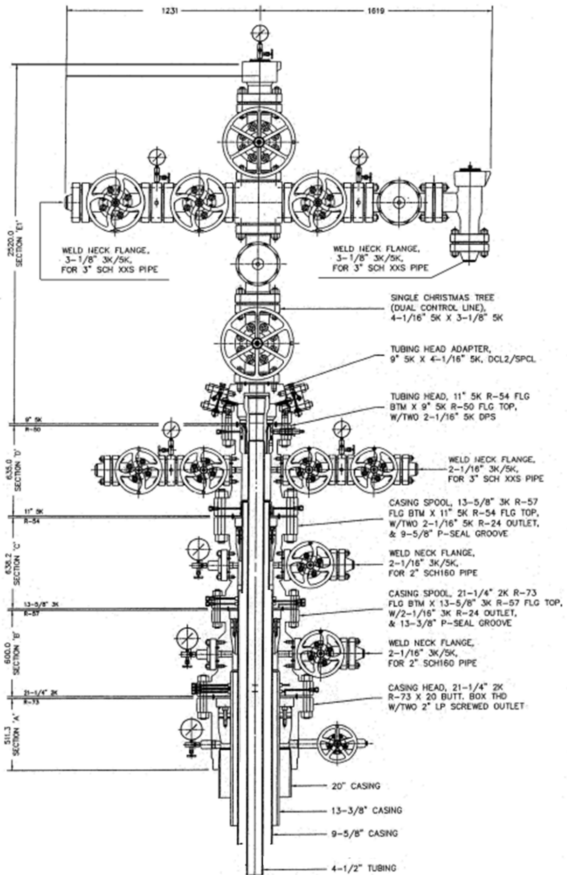
Fig 2: Schematic of wellhead and X-mas tree
