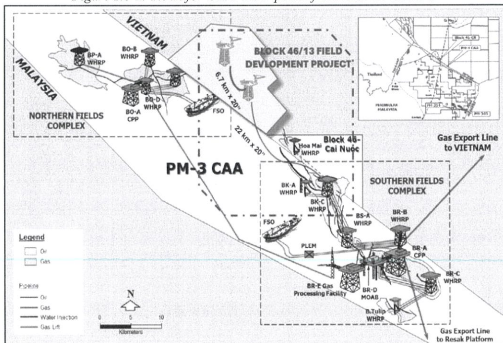
Figure 1.0-2: Tie In for Gas FWS Pipeline from KM/DD to BK-C
