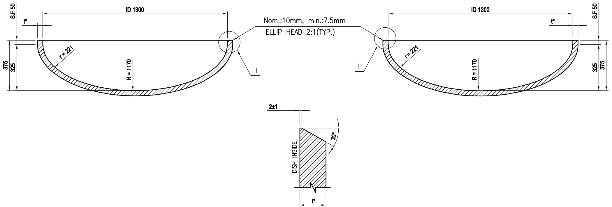
DETAIL I
