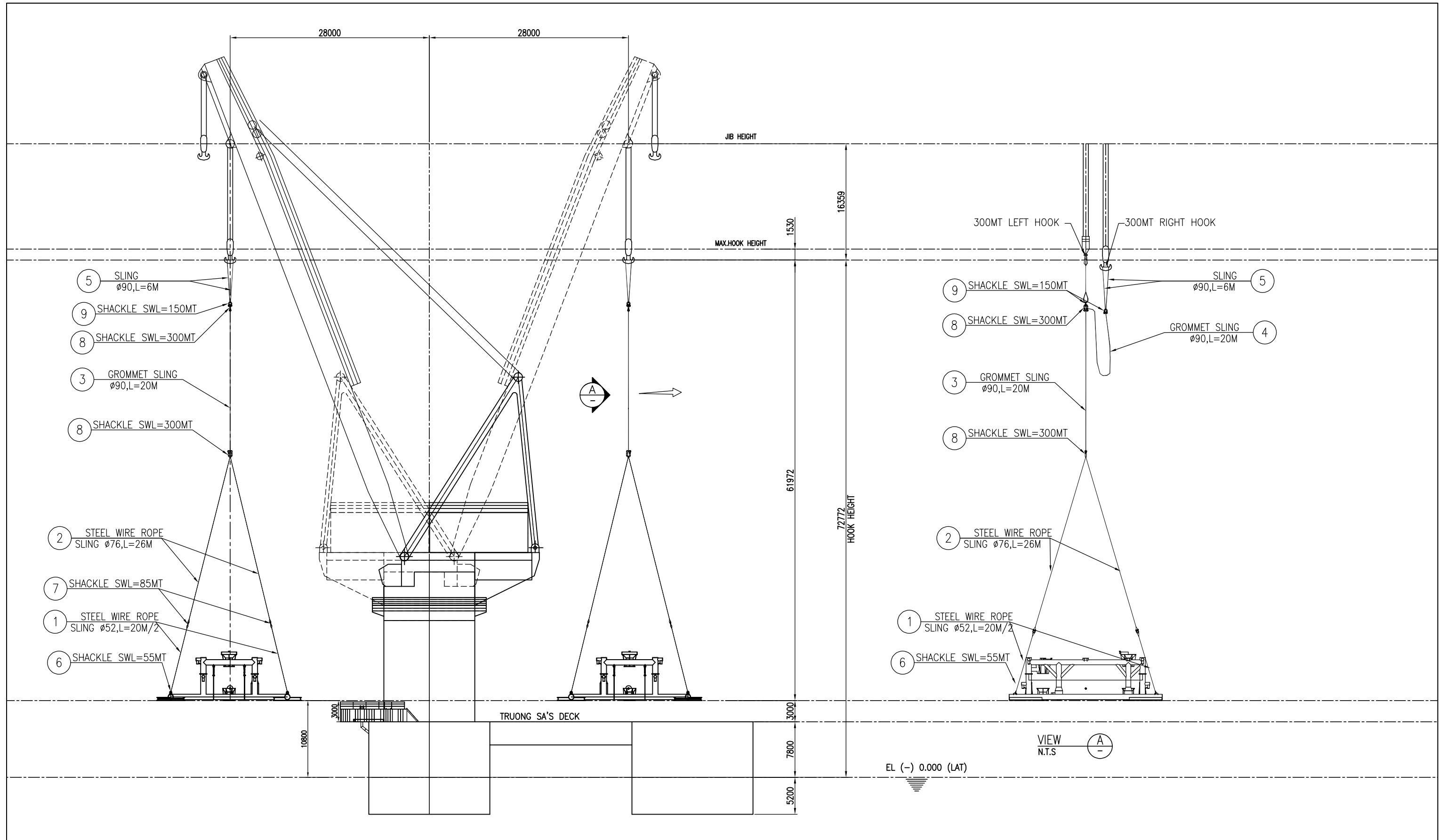
LIFTING ARRANGEMENT FOR SUBSEA TEMPLATE
