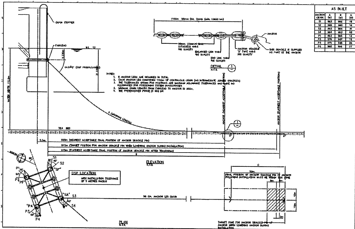
Mooring chain layout
