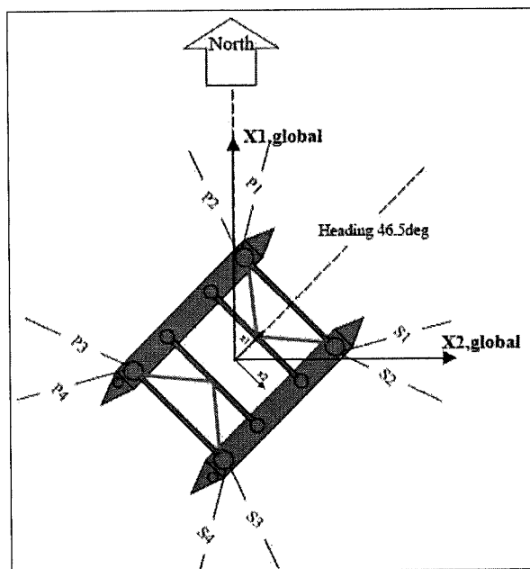
Anchor system layout
