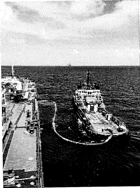
Start to transfer hose string to export tanker
