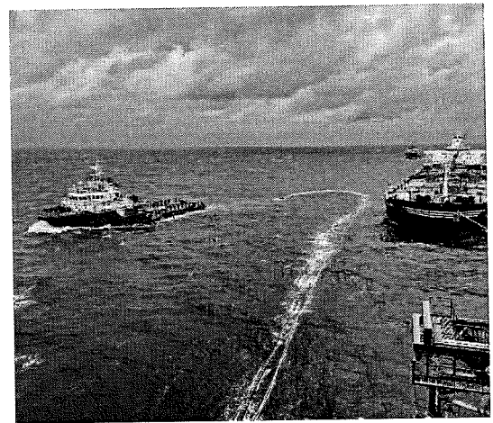
Recover the hosetring after lifting operation
