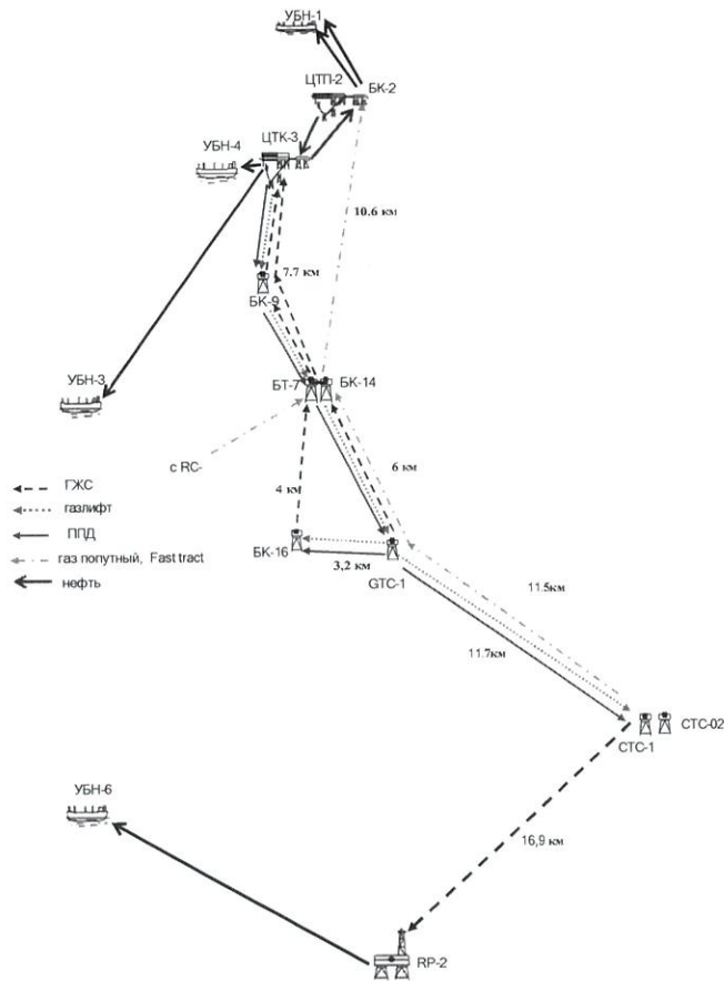
Figure 1: Location of CTC1 and CTC2 Wellhead Platforms at Ca Tam Field
