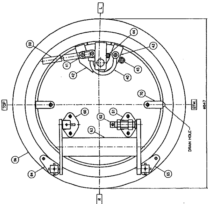
FRONT VIEW (HORIZONTAL w/HINGE)
