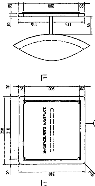
BRACKET SCALE 1:5
