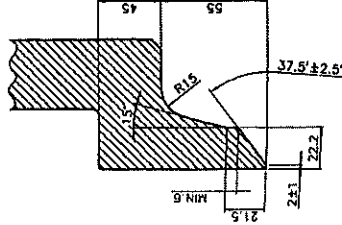
DETAIL OF HUB END (SEE NOTE 3.)
