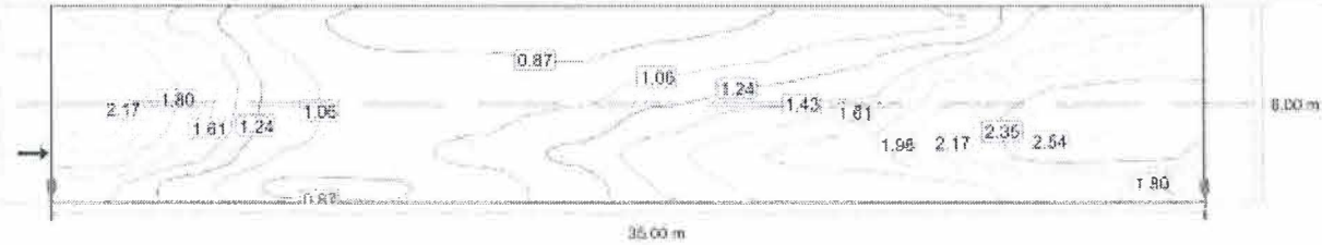
Observer 1: Maintenance value, luminance with dry roadway [cd/m²] (Iso-illuminance curves)
