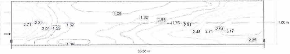
Observer 1: Luminance with new installation [cd/m²] (Iso-illuminance curves)
