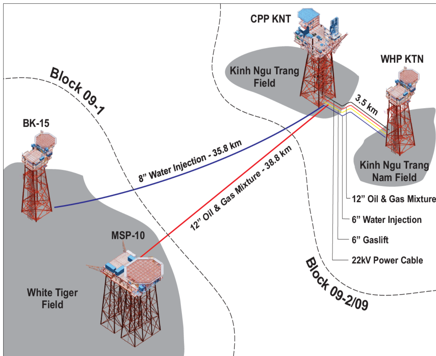
Figure 1: Scheme of Kinh Ngu Trang and Kinh Ngu Trang Nam field
