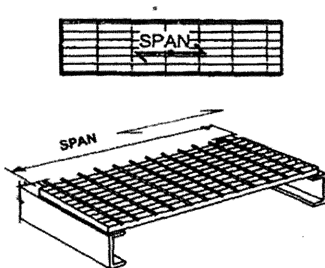
Fig.5: The Grating (Galv.)
