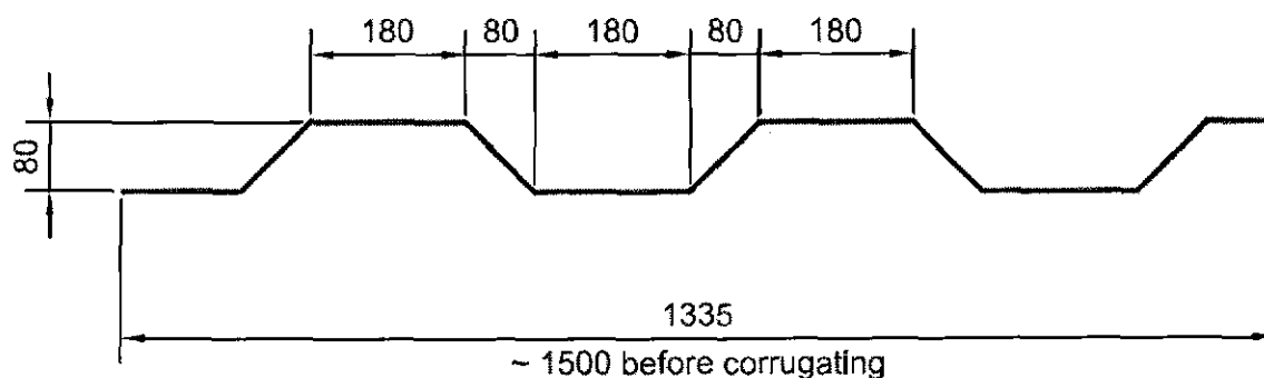
Fig.3: The 10mm THK Fire wall Profile
