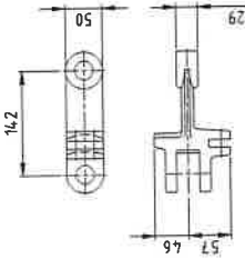
special forged chain link for scraper
