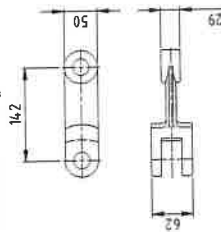
standard forged chain link
