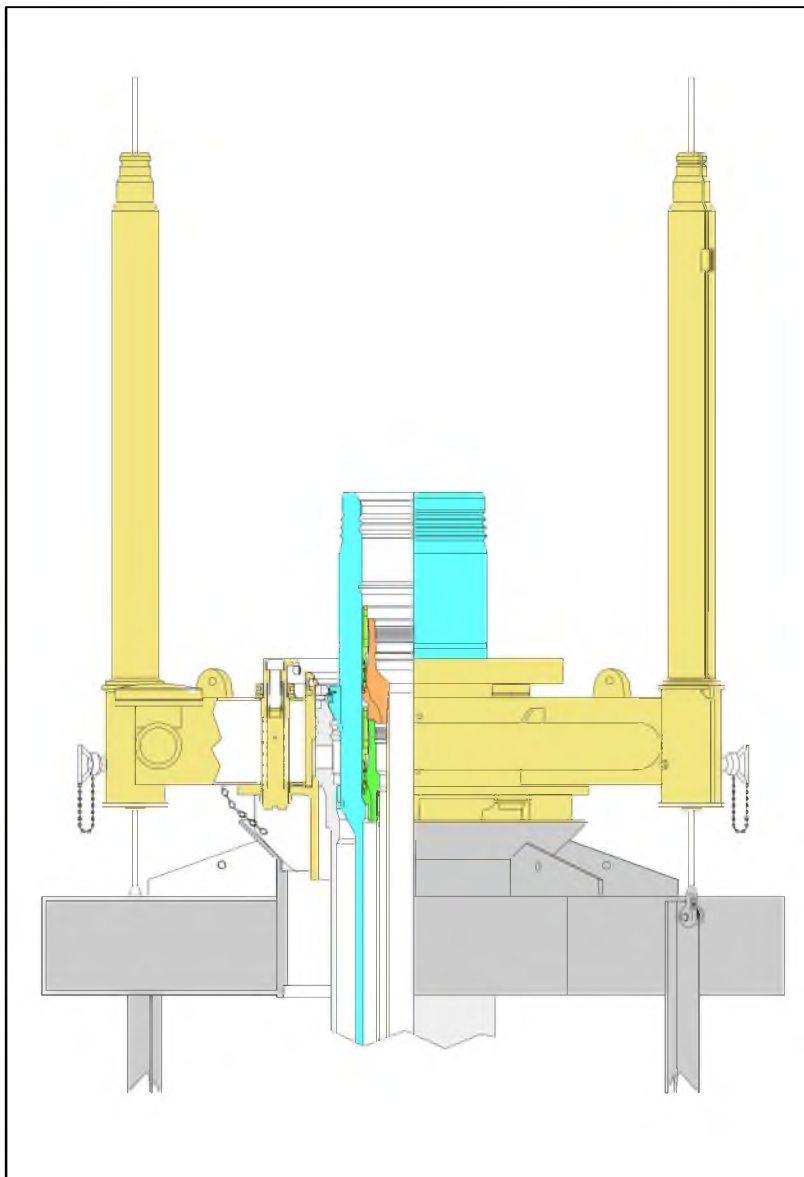
SG-5 Wellhead System Stackup
