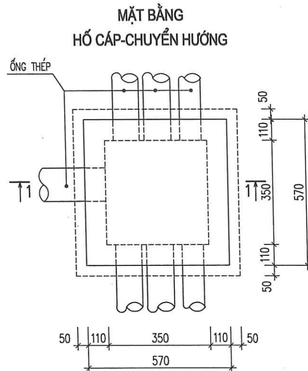
TĐ1 570X570X100
