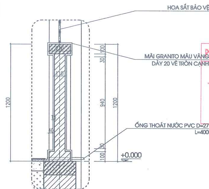
LAN CAN LC1-8 (SL: 02CK; L=3380) LAN CAN LC1-9 (SL: 01CK; L=3680)
