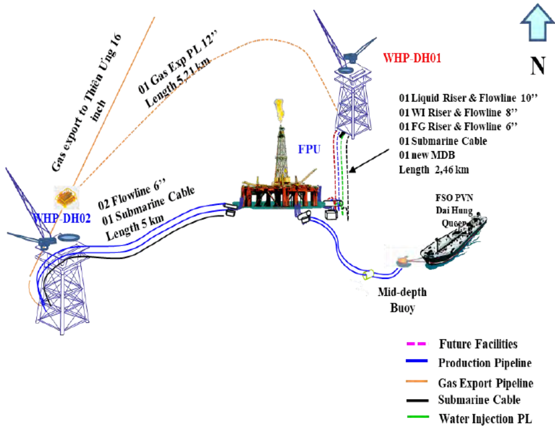
Figure 1: Dai Hung Overall Field Layout
