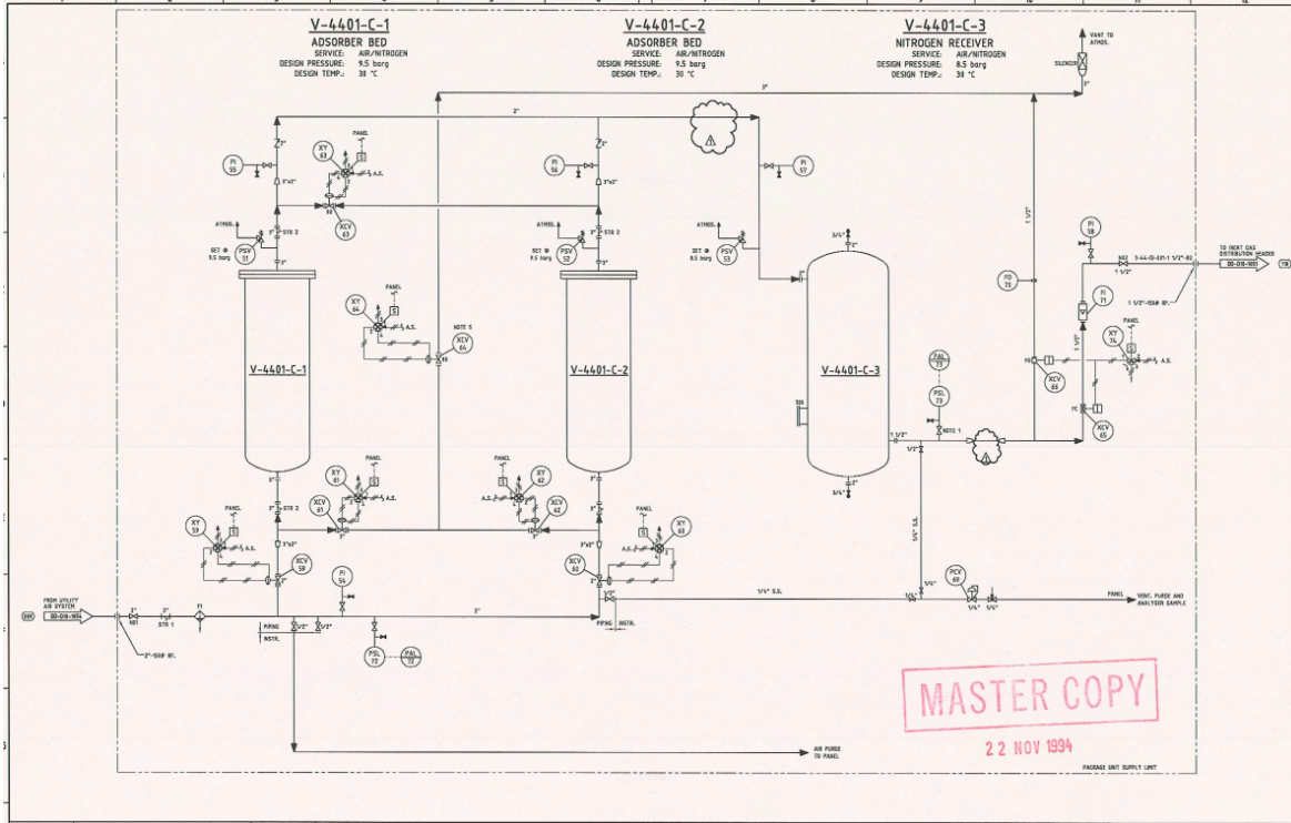
Figure 2: P&I Diagram - Nitrogen System on DH-01 FPU
