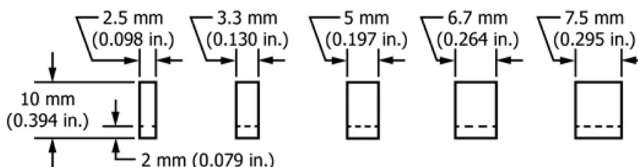
(a) Standard Full Size Specimen
