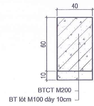
CẮT IV - IV (1/25)
