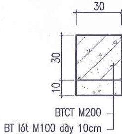
CẮT III - III (1/25)
