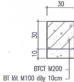
CẮT V - V (1/25)
