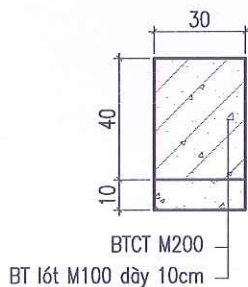
CẮT II - II (1/25)
