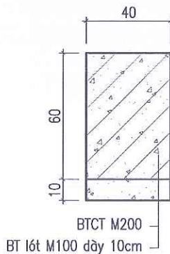
CẮT IV - IV (1/25)
