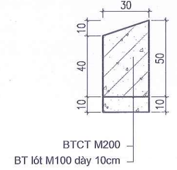
CẮT V - V (1/25)
