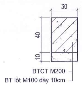
CẮT II - II (1/25)
