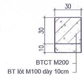
CẮT III - III (1/25)
