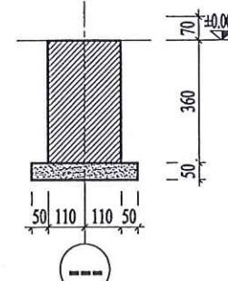
MC 3-3
