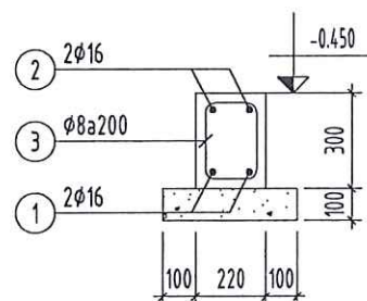
GIANG GM5 (SL= 02, L= 1.670m)
