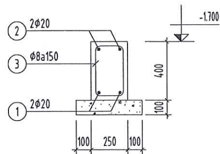
GIANG GM1 (SL= 02, L= 9.920m)
