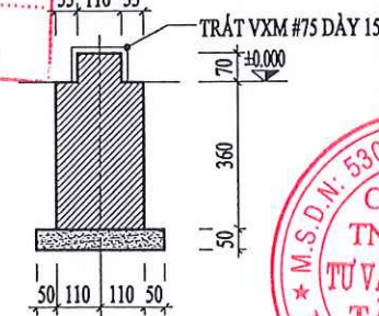
MC 2-2
