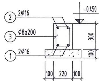
GIANG GM6 (SL= 02, L= 6.270m)
