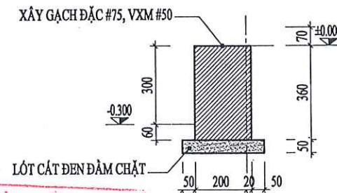
MC 1-1
