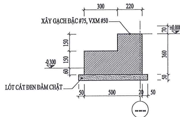
MC 4-4
