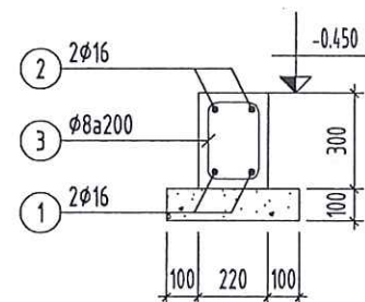
GIANG GM5 (SL= 02, L= 6.270m)
