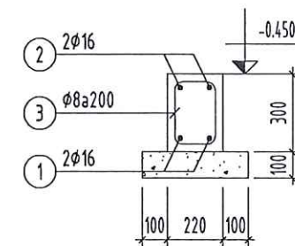
GIANG GM4 (SL= 01, L= 2.670m)
