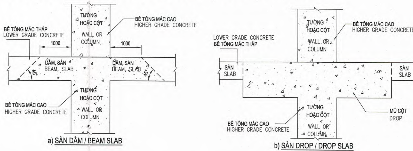
b) SÀN DROP / DROP SLAB
