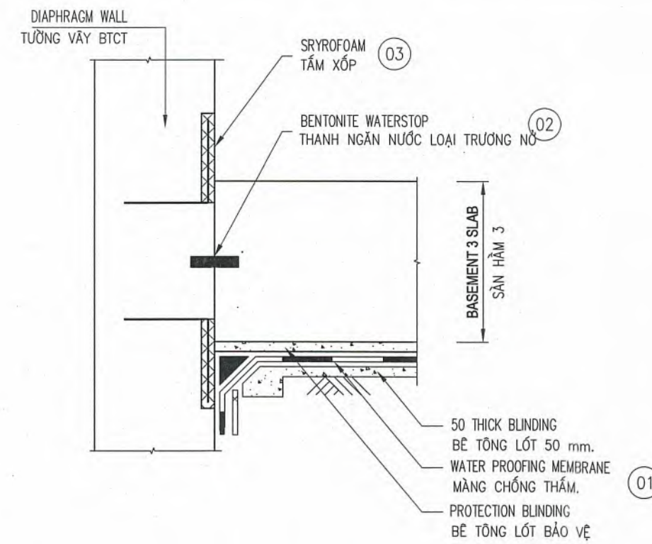
1. WALL/SLAB ON GRADE JOINT DETAIL
